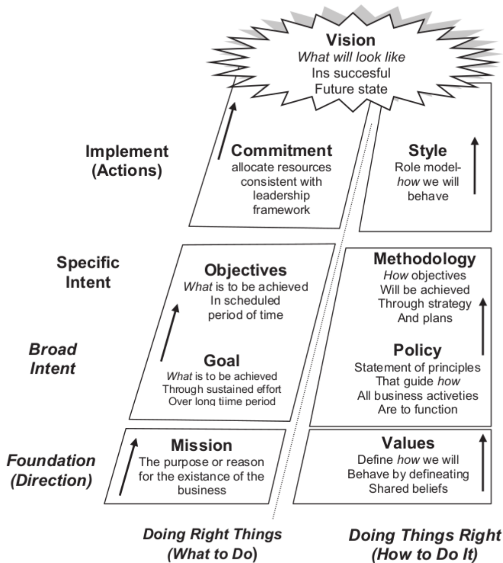
Gambar 3. Leadership Framework
