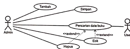
Gambar 4. Use Case Diagram Data Buku
