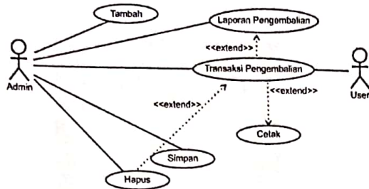
Gambar 6. Use Case Diagram Data
