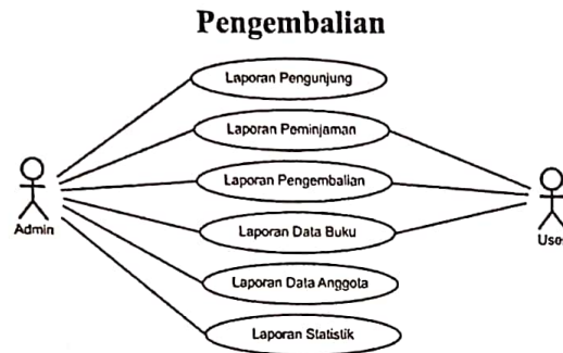
Gambar 7. Use Case Diagram Data Laporan
